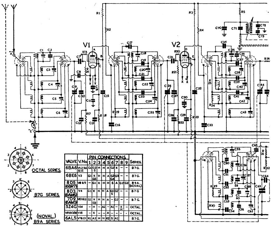
CIRCUIT DIAGRAM—
