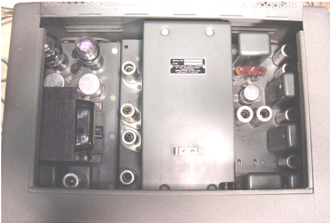
Above: beneath chassis view with coilbox cover in place. Below: above-chassis 'peephole' view through the access 'lid'
